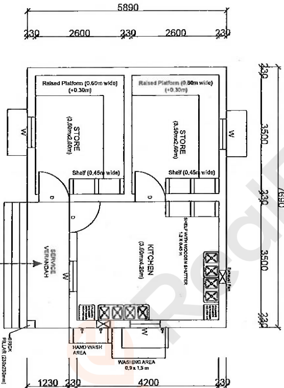
PLAN-5 (501 - 600 STUDENTS)
