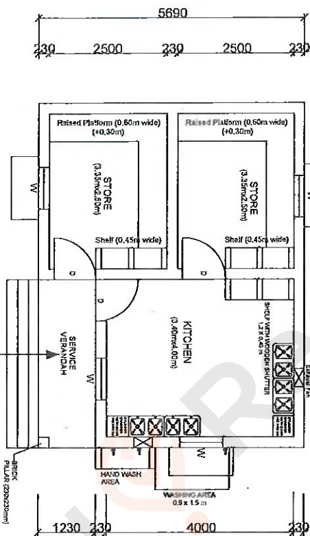
PLAN-4 (401 - 500 STUDENTS)
