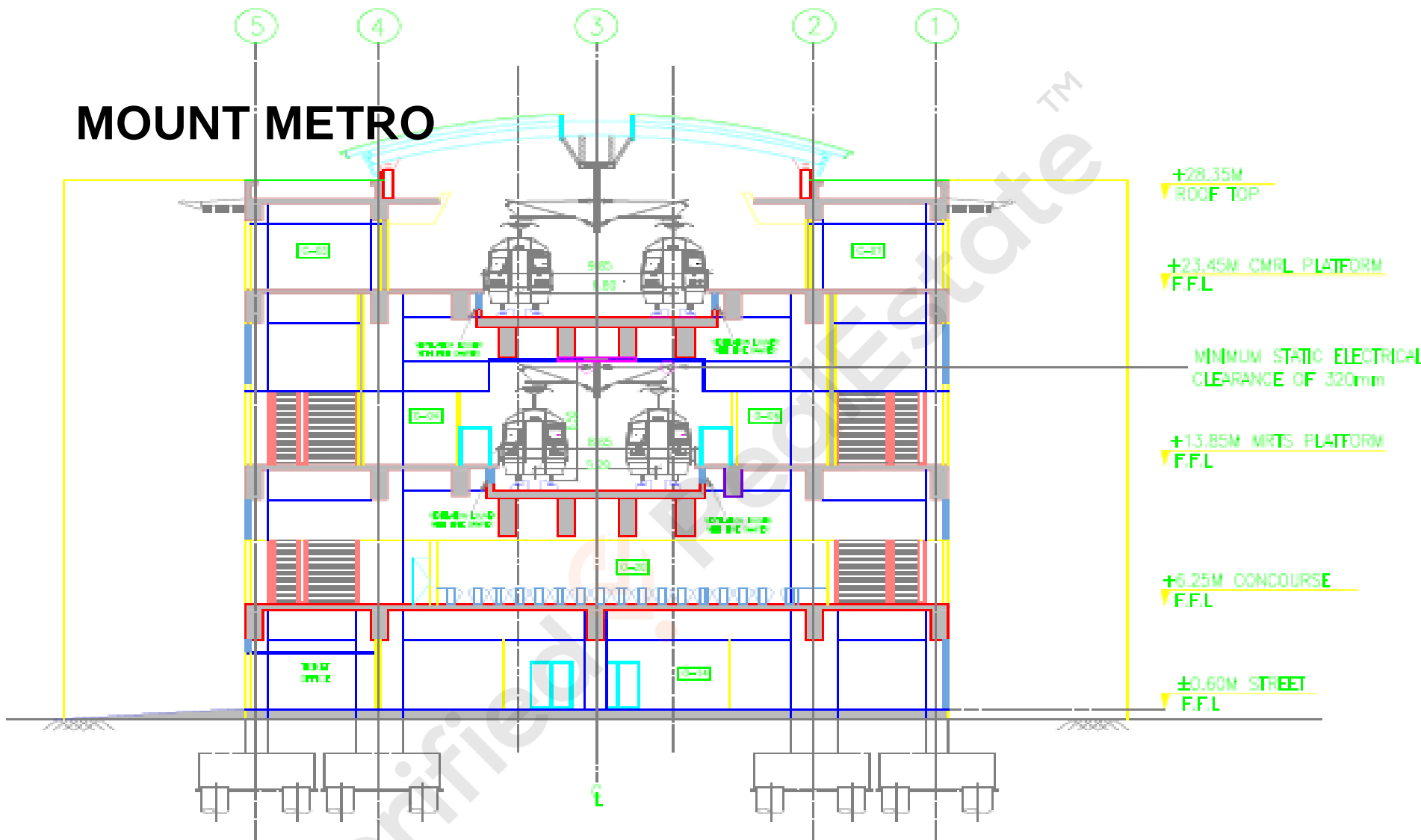
ST. THOMAS MOUNT MID STATION SECTION DRAWING
