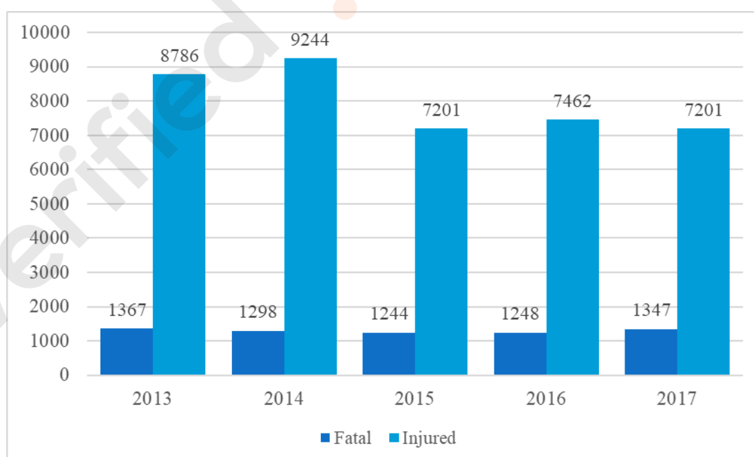
Figure 2-19 Accident Data 2013-17
