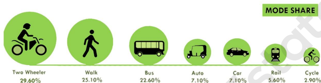
Figure 3: Modal Share
