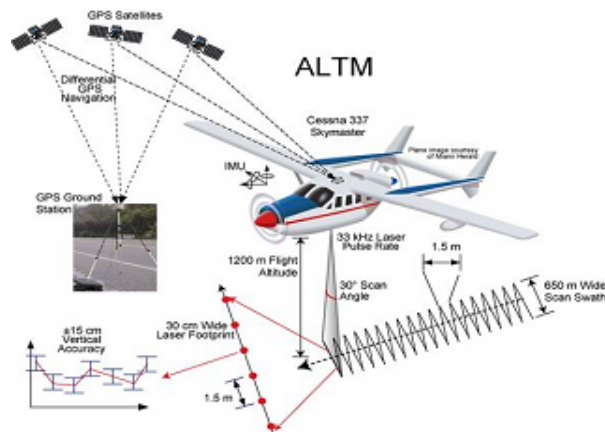
Airborne Laser Terrain Mapping (ALTM)
